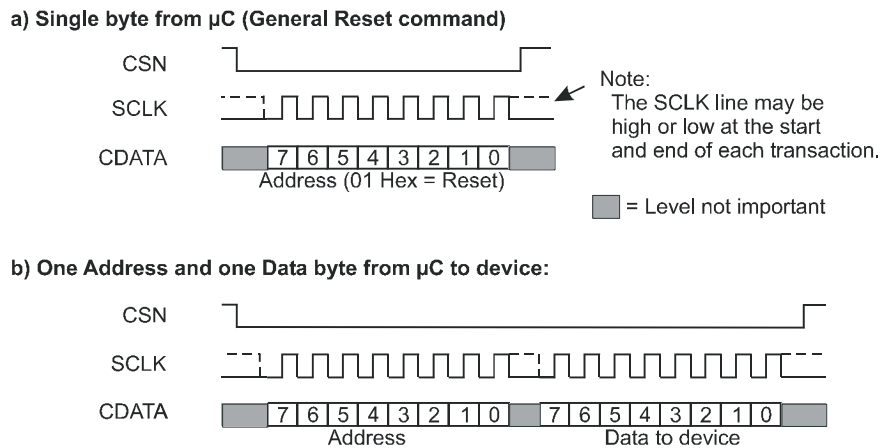
Figure 8 C-BUS Transactions
