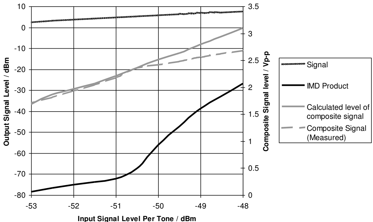
Figure 13 Variations in Signal and IMD Product Levels
