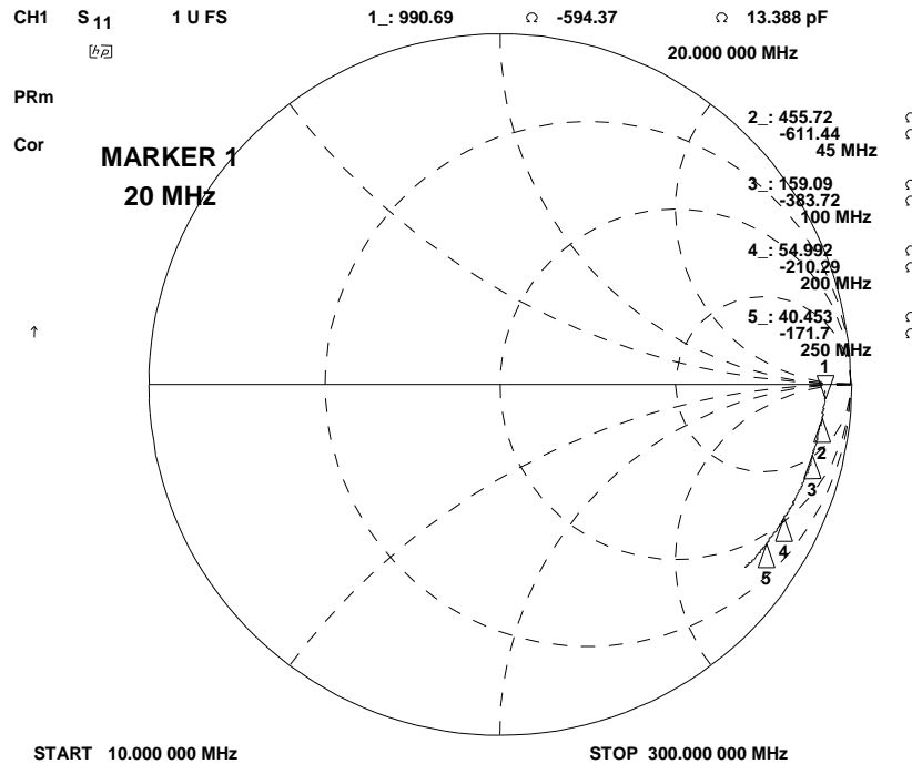
Figure 9 Quadrature Demodulator Input Impedance
