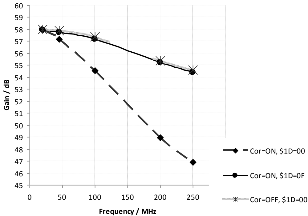
Figure 6 Frequency Response, showing effect of COR bit ($1C, b6) and FREQ bits($1D, b3-b0)
