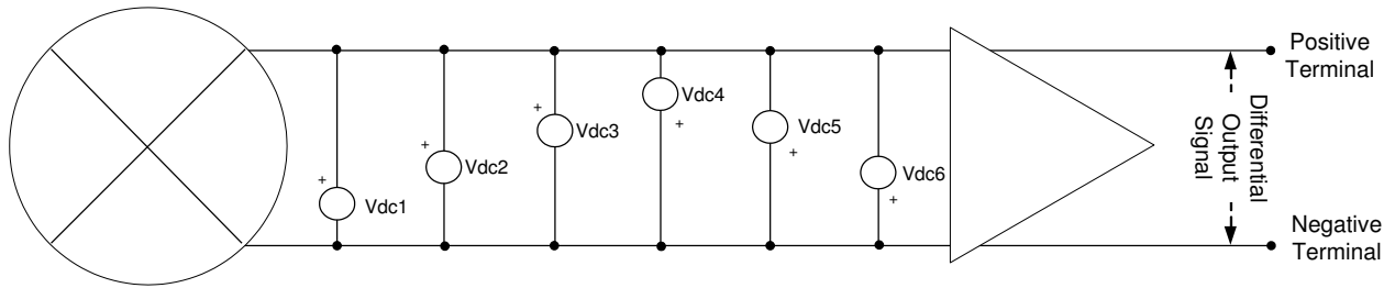
Figure 7 Simplified Schematic of DC Offset Correction
