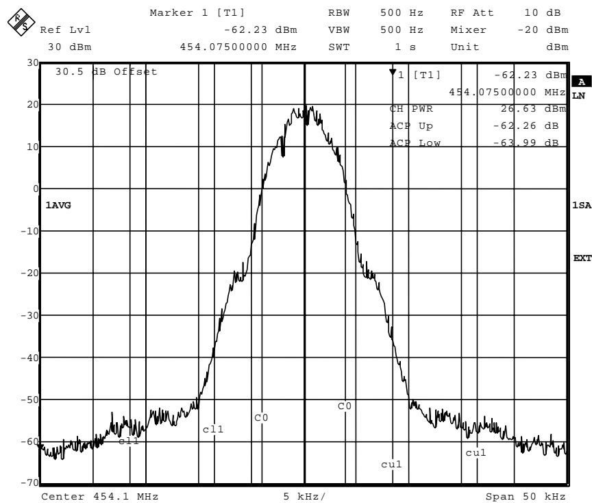
Figure 37 TX ACP of -62dBc (12.5kHz channel settings) at +30dBm carrier, 8kbps, BT = 0.27, IF 90MHz
