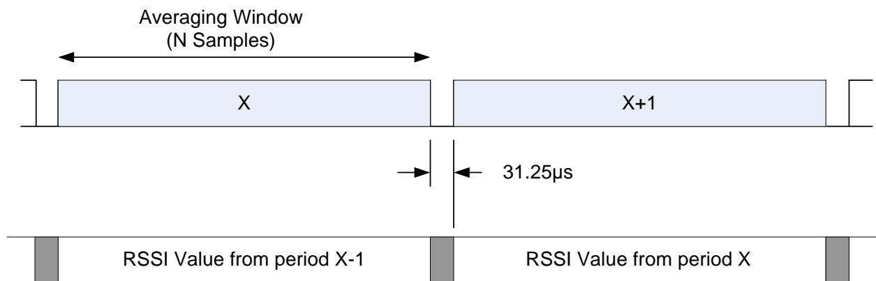
Figure 25 RSSI Timing
