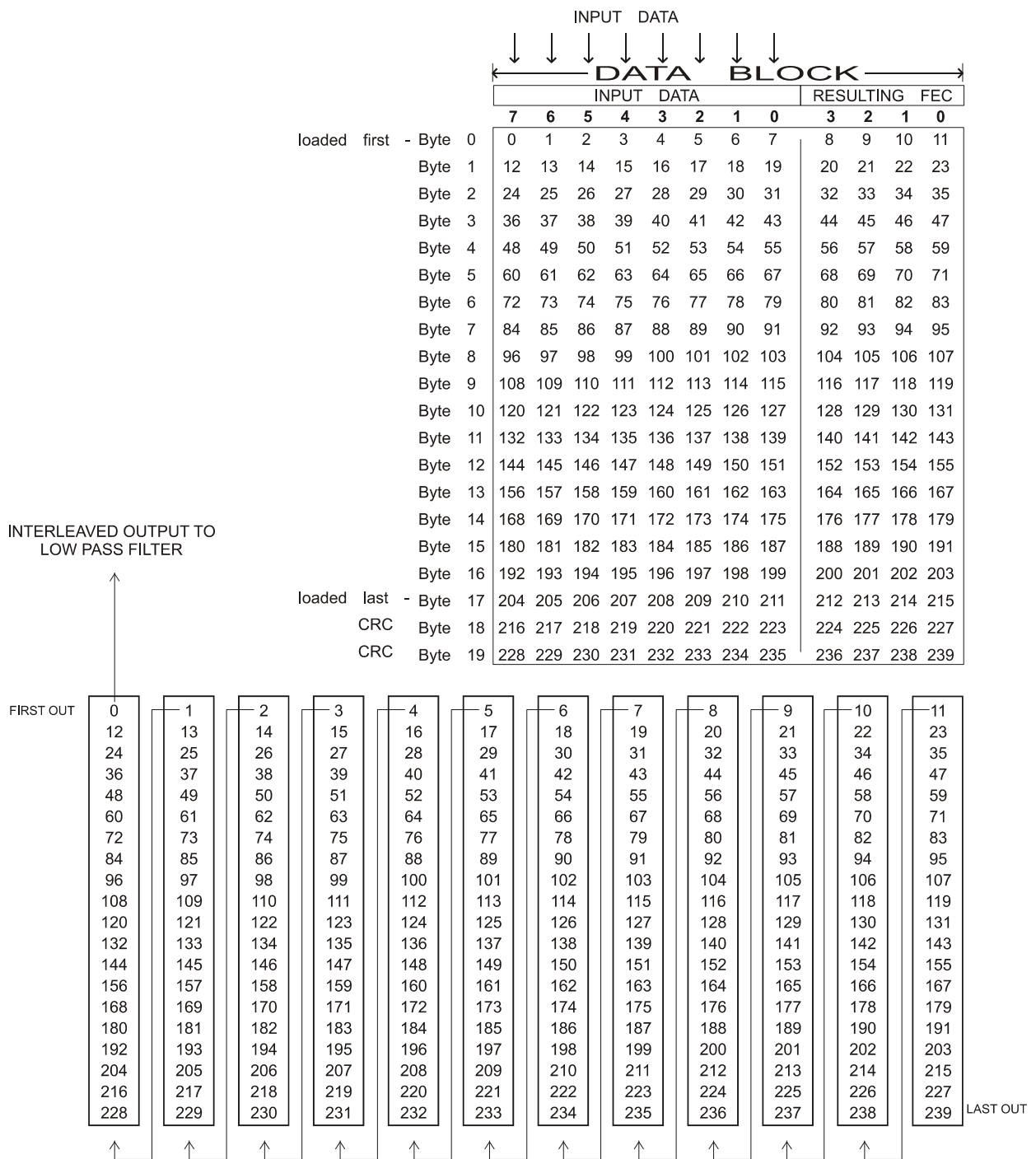
Figure 26 Interleaving - Input/Output
