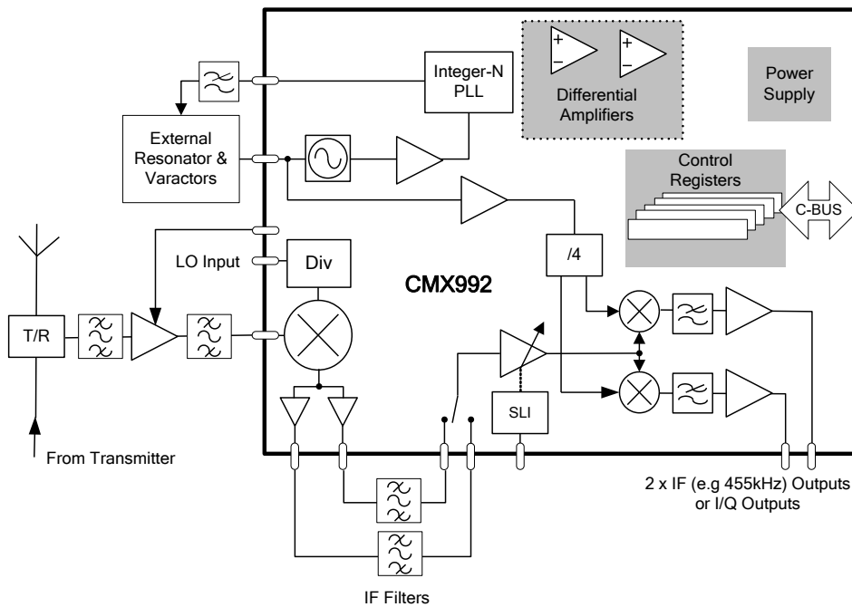
Figure 2 CMX992 – RF Quadrature/Low IF Receiver
