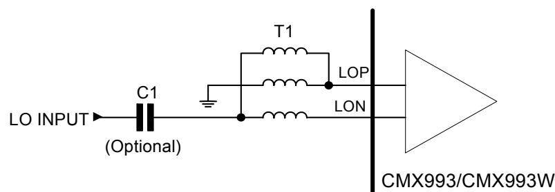
Figure 5 LO Input Configuration using a 1:1 Balun (60MHz to 2GHz)
