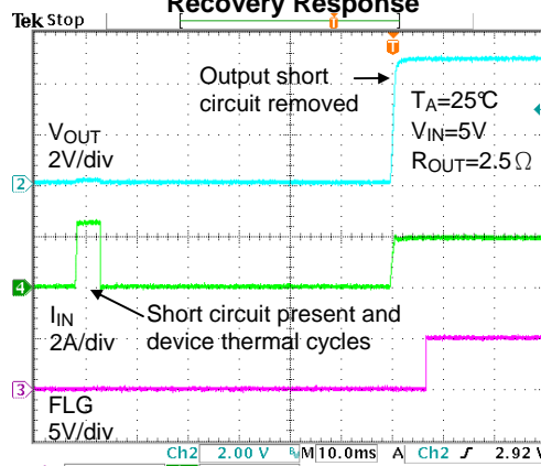
Short-Circuit to Full-Load Recovery Response
