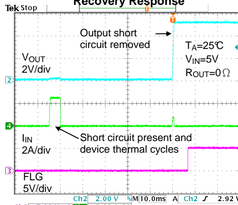
Short-Circuit to No-Load Recovery Response
