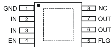
MSOP-8 /MSOP-8EP Note: latter with exposed pad (dotted line)
