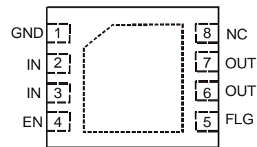
U-DFN3030-8 Type E
