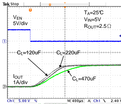
Inrush Current
