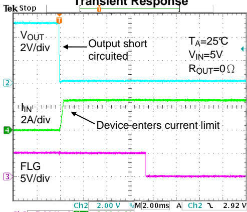
No-Load to Short-Circuit Transient Response
