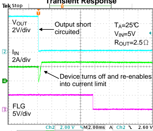
Full-Load to Short-Circuit Transient Response
