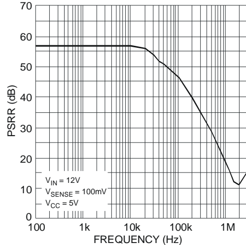
Fig. 19 Supply Rejection
