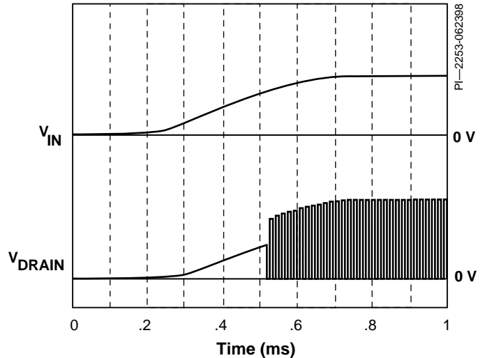
Figure 7. TinySwitch Power-Up Timing Diagram.
