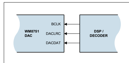
Figure 13 Slave Mode
