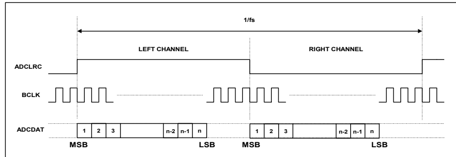
Figure 13 Left Justified Mode
