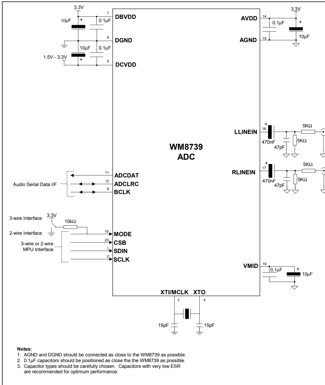
Figure 29 External Components Diagram
