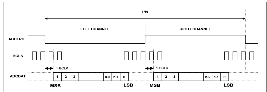
Figure 14 I^2S Mode
