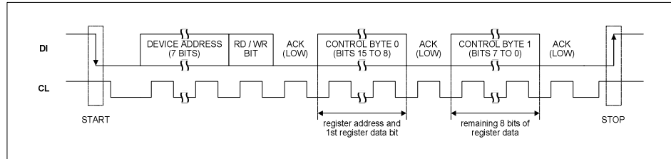
Figure 21 2-wire Serial Interface
