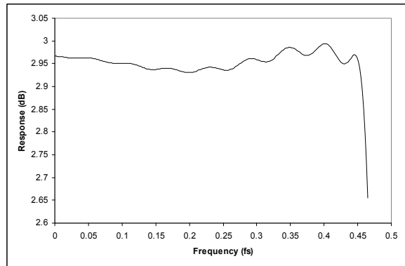
Figure 44 DAC Digital Filter Ripple (64xOSR)
