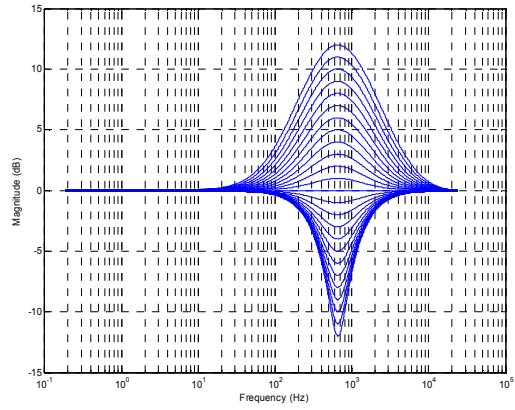
Figure 56 EQ Band 3 – Peak Filter Centre Frequencies, EQ3| Figure 57 EQ Band 3 – Peak Filter Gains for Lowest Cut-off Frequency, EQ3BW=0
