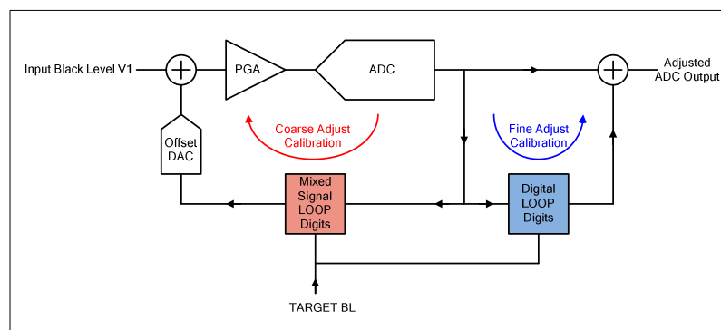
Figure 23 BLC Top-Level Circuitry
