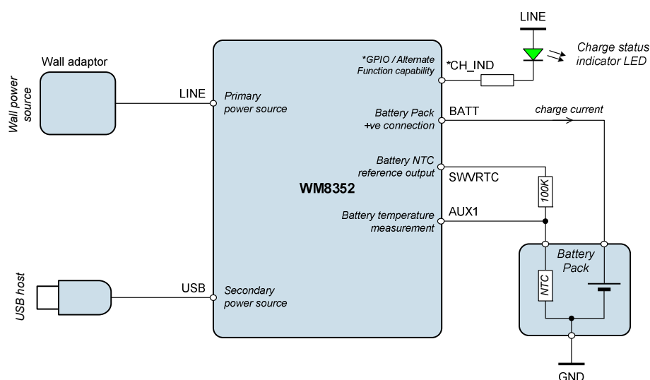
Figure 76 Typical Connections for WM8352 Battery Charger
