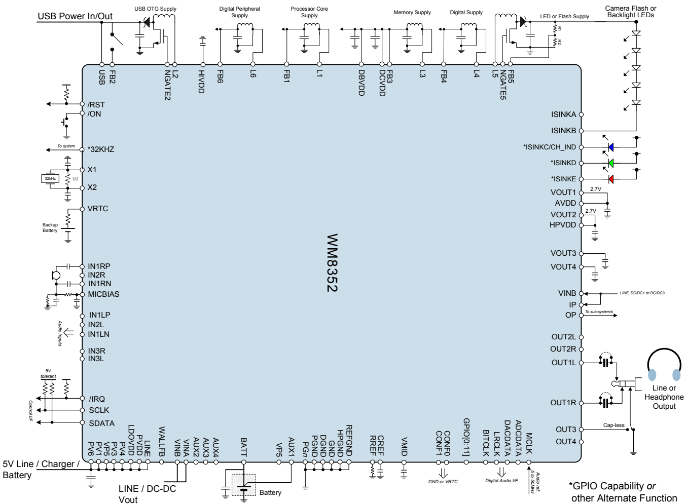
Figure 87 WM8352 Typical Connections Diagram
