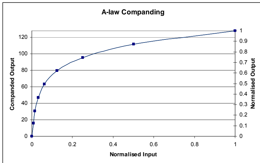
Figure 29 A-Law Companding
