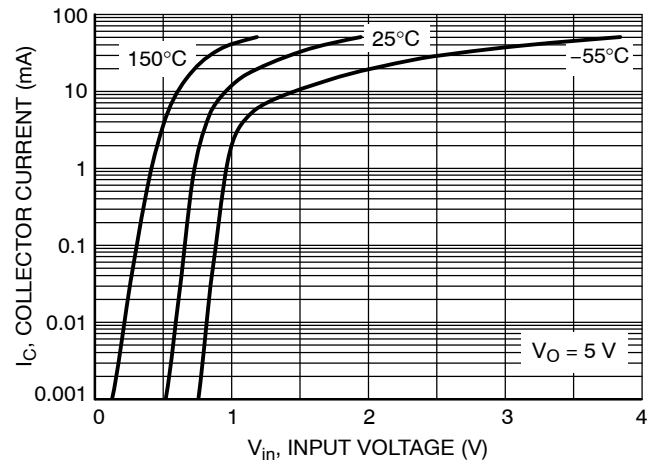
Figure 30. Output Current vs. Input Voltage
