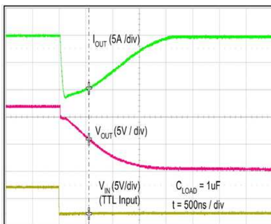
Figure 42. Quasi-Static Sink Current with V_{DD}=12V^{(13)}
