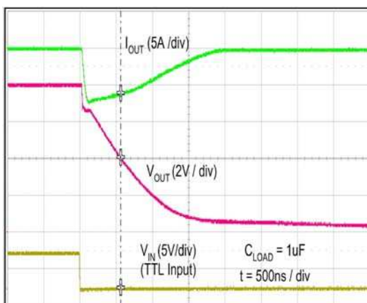
Figure 44. Quasi-Static Sink Current with V_{DD}=8V^{(13)}
