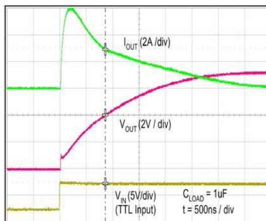
Figure 43. Quasi-Static Source Current with V_{DD}=8V^{(13)}
