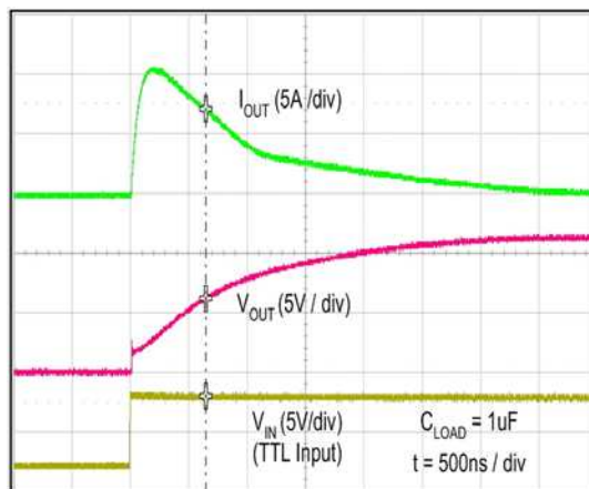
Figure 41. Quasi-Static Source Current with V_{DD}=12V^{(13)}
