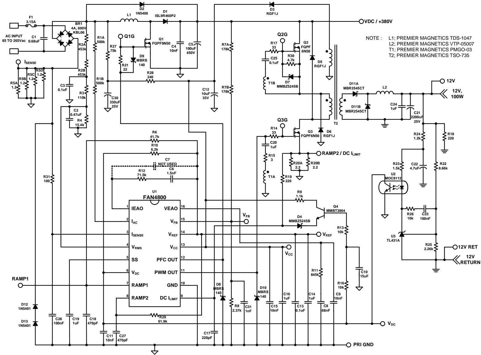
Figure 13. Voltage-Mode Application
