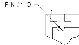
OPTIONS OF PIN ONE IDENTIFIERS
