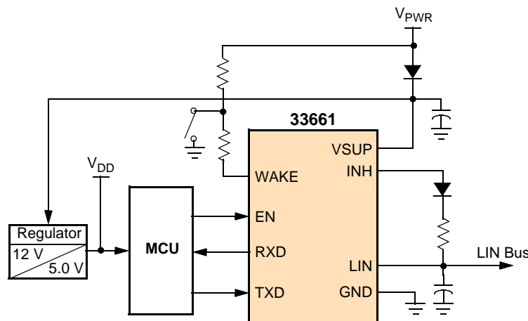
Figure 1. 33661 Simplified Application Diagram
