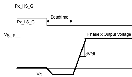
Figure 17. Positive dV/dt Transient
