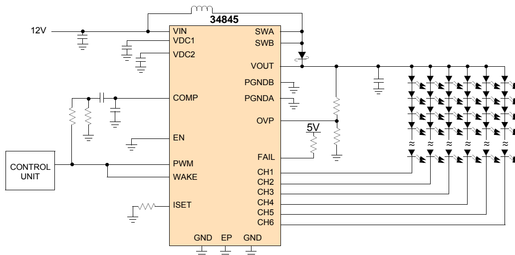
Figure 1. 34845 Simplified Application Diagram
