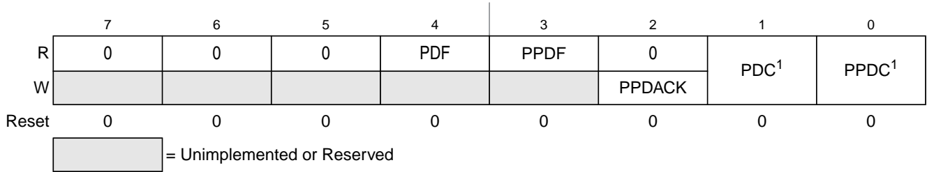
Figure 5-11. System Power Management Status and Control 2 Register (SPMSC2)
