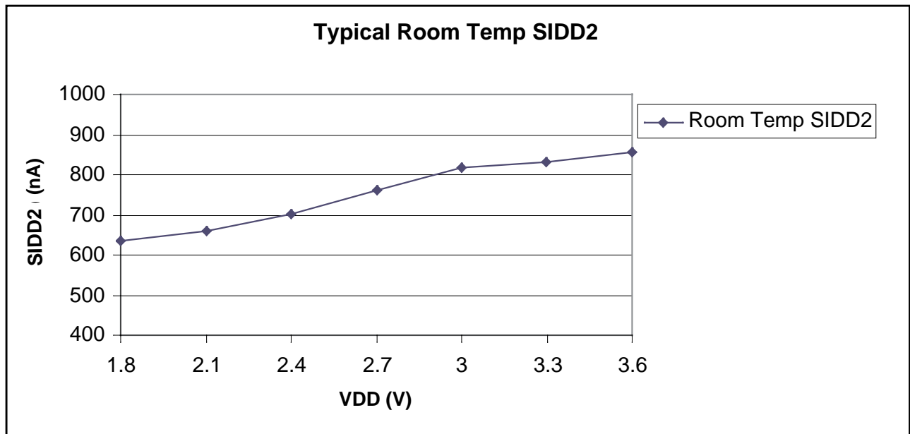
Figure A-8. Typical Stop 2 I DD
