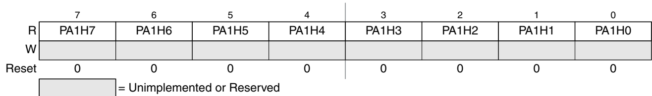
Figure 14-55. 8-Bit Pulse Accumulators Holding Register 1 (PA1H)
