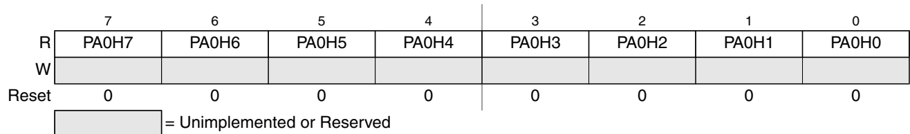
Figure 14-56. 8-Bit Pulse Accumulators Holding Register 0 (PA0H)
