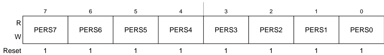
Figure 19-31. Port S Pull Device Enable Register (PERS)
