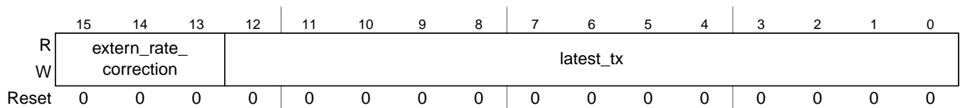
Figure 13-86. Protocol Configuration Register 21 (PCR21)
