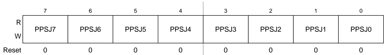
Figure 19-64. Port J Polarity Select Register (PPSJ)
