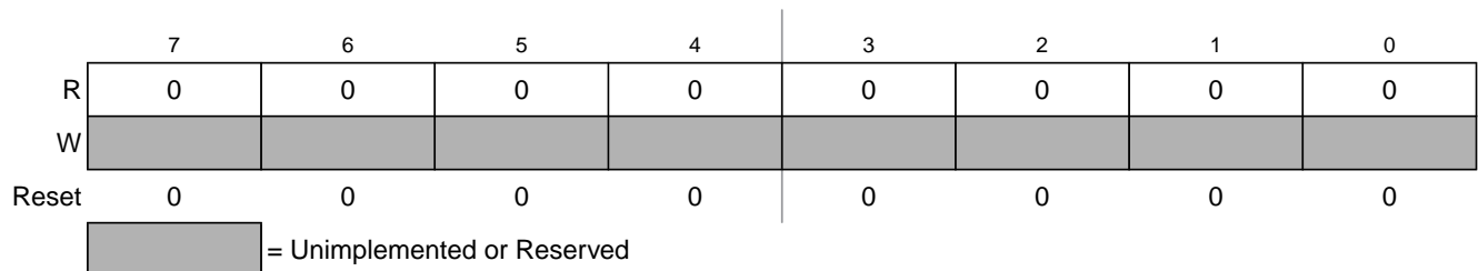
Figure 19-66. PIM Reserved Register
