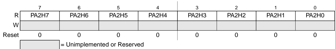
Figure 26-54. 8-Bit Pulse Accumulators Holding Register 2 (PA2H)
