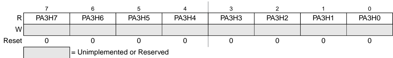
Figure 26-53. 8-Bit Pulse Accumulators Holding Register 3 (PA3H)
