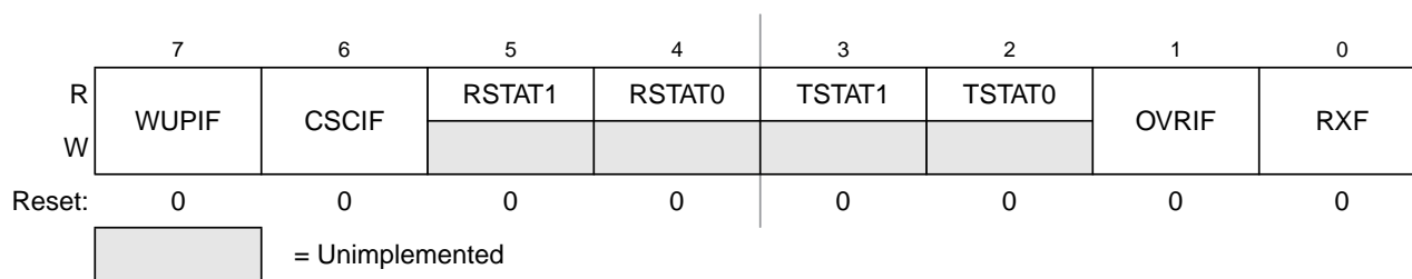
Figure 21-8. MSCAN Receiver Flag Register (CANRFLG)
