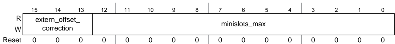
Figure 13-94. Protocol Configuration Register 29 (PCR29)
