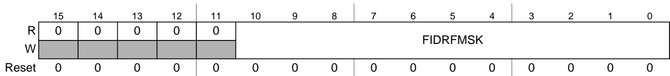
Figure 13-60. Receive FIFO Frame ID Rejection Filter Mask Register (RFFIDRFMR)
