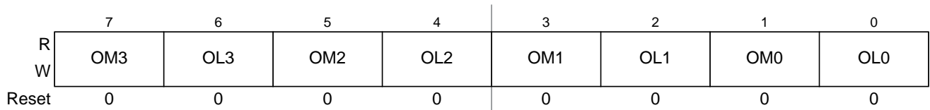
Figure 26-12. Timer Control Register 2 (TCTL2)
