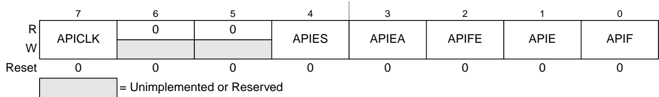
Figure 3-3. Autonomous Periodical Interrupt Control Register (VREGAPICL)
