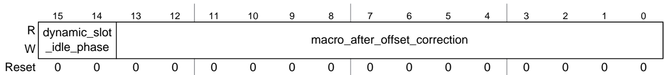
Figure 13-93. Protocol Configuration Register 28 (PCR28)
