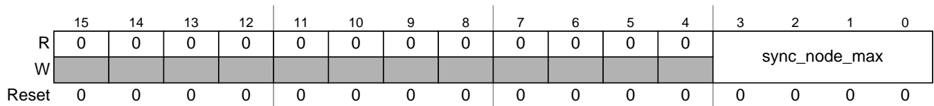
Figure 13-95. Protocol Configuration Register 30 (PCR30)
