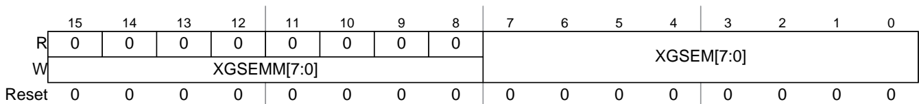
Figure 14-12. XGATE Semaphore Register (XGSEM)
