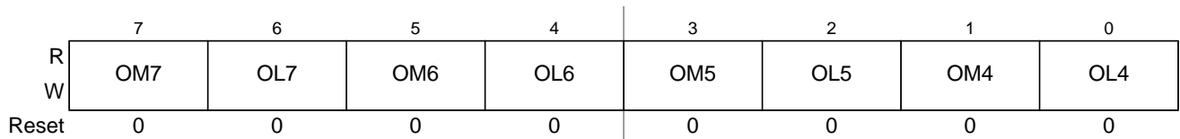
Figure 26-11. Timer Control Register 1 (TCTL1)
