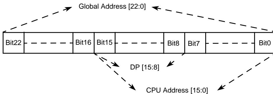
Figure 11-9. DIRECT Address Mapping
