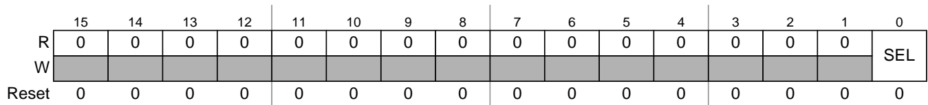
Figure 13-52. Receive FIFO Selection Register (RFSR)
