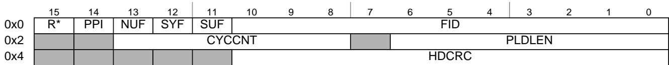
Figure 13-105. Frame Header Structure
