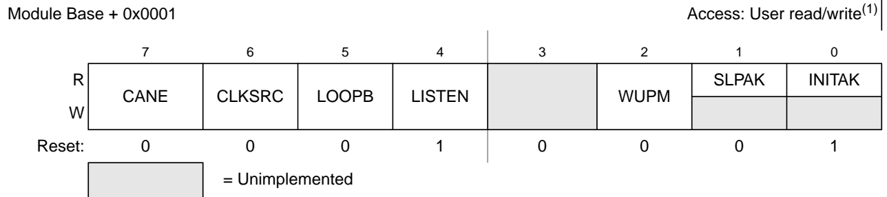
Figure 21-5. MSCAN Control Register 1 (CANCTL1)
