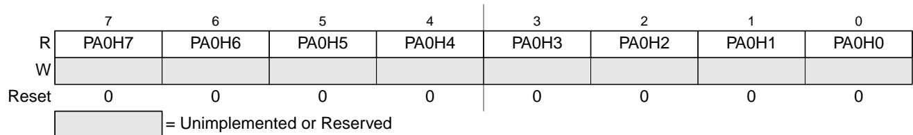
Figure 26-56. 8-Bit Pulse Accumulators Holding Register 0 (PA0H)
