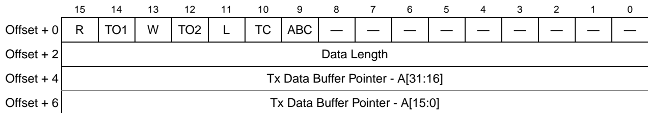
Figure 17-26. Transmit Buffer Descriptor (TxBD)
