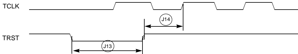
Figure 24. \overline{TRST} Timing
