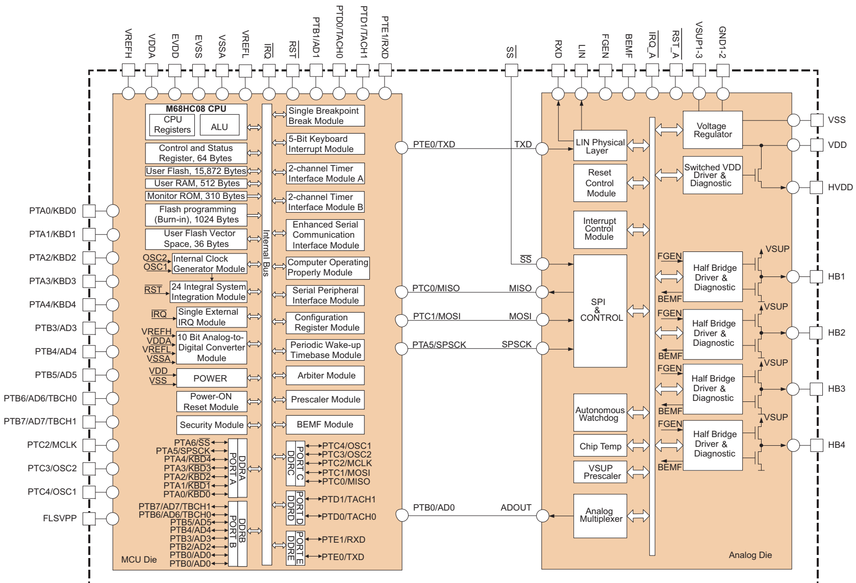
Figure 2. 908E626 Simplified Internal Block Diagram
