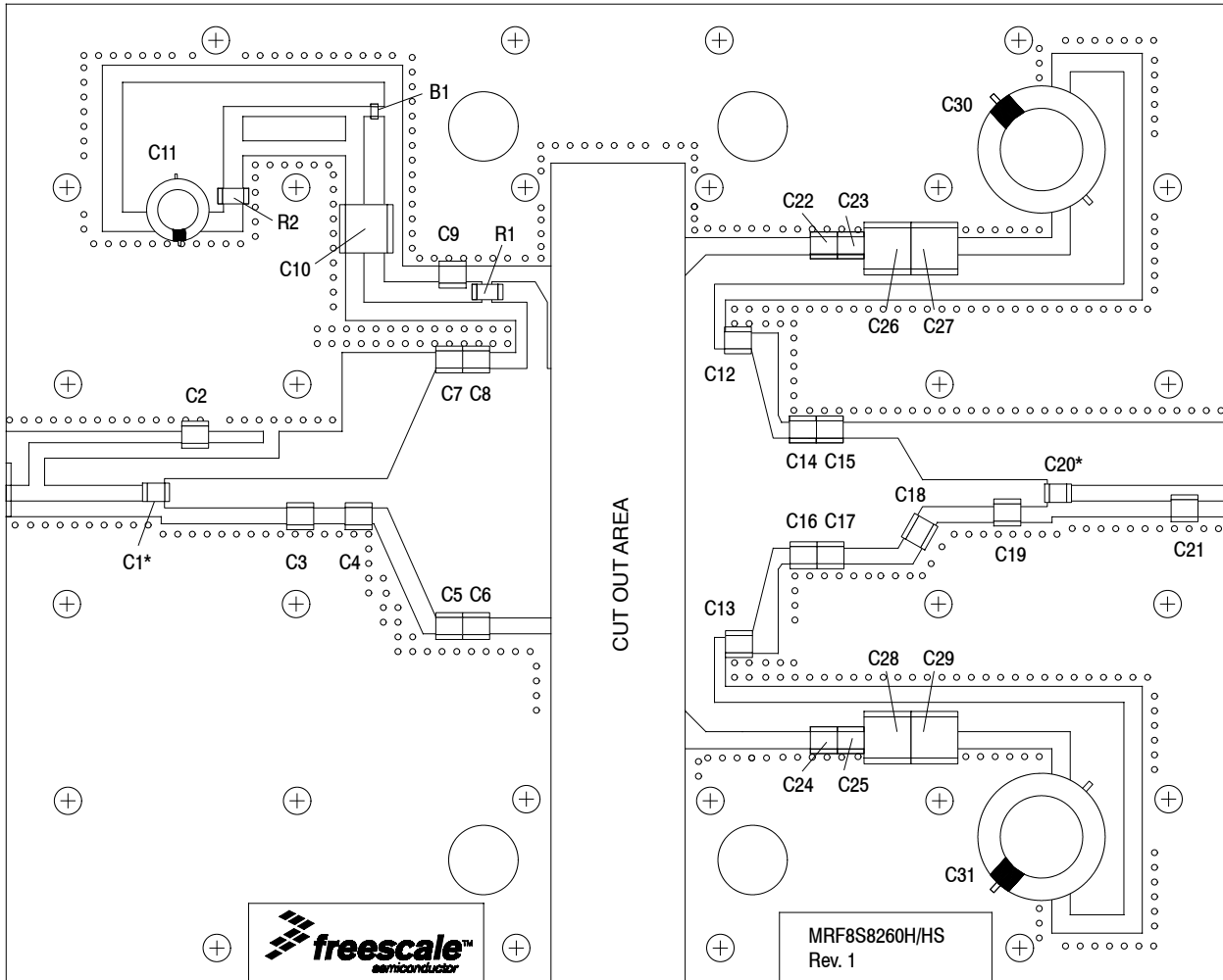
Figure 1. MRF8S8260HR3(HSR3) Test Circuit Component Layout
