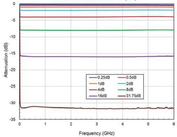
Normalized Attenuation (dB)
