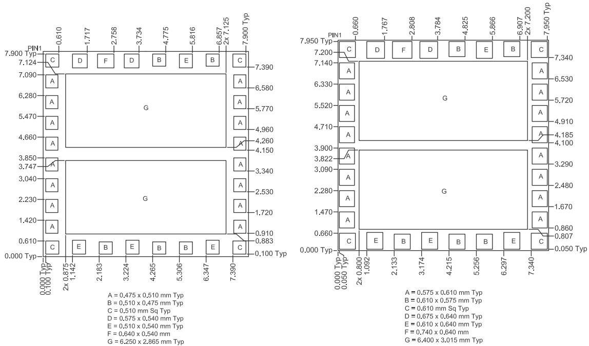
PCB MET/L LAND PATTERN
