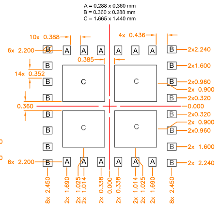
PCB Stencil Pattern
