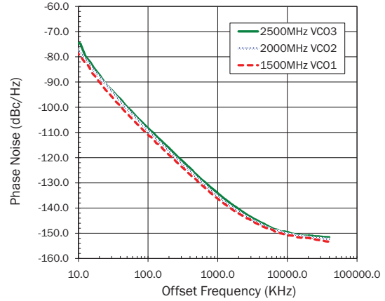
VCO Phase Noise With LO Divide by 2
