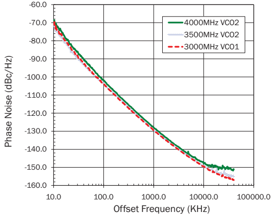
VCO Phase Noise With LO Divide by 1
