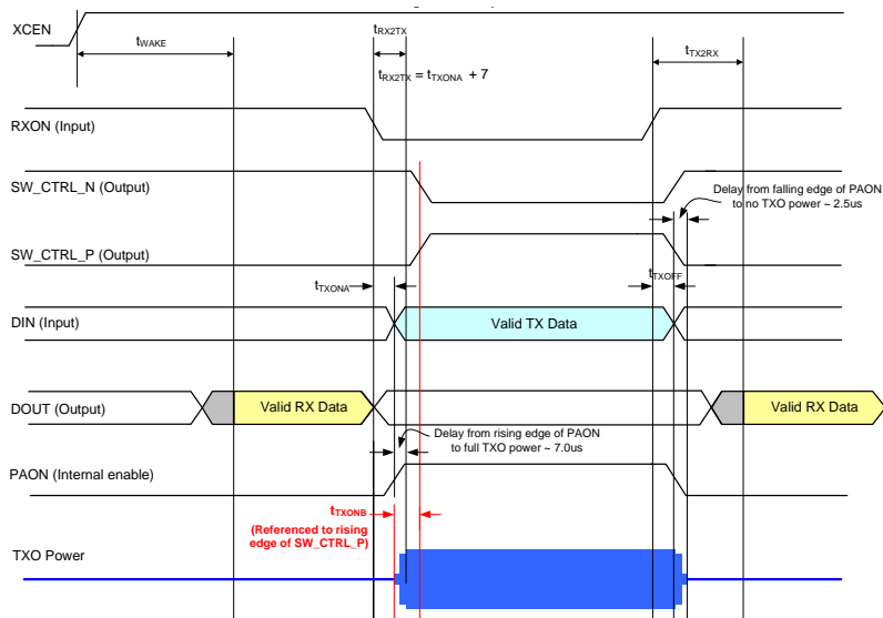
Figure 2b: Control Timing for TDD Operation, PAFIRST=1
