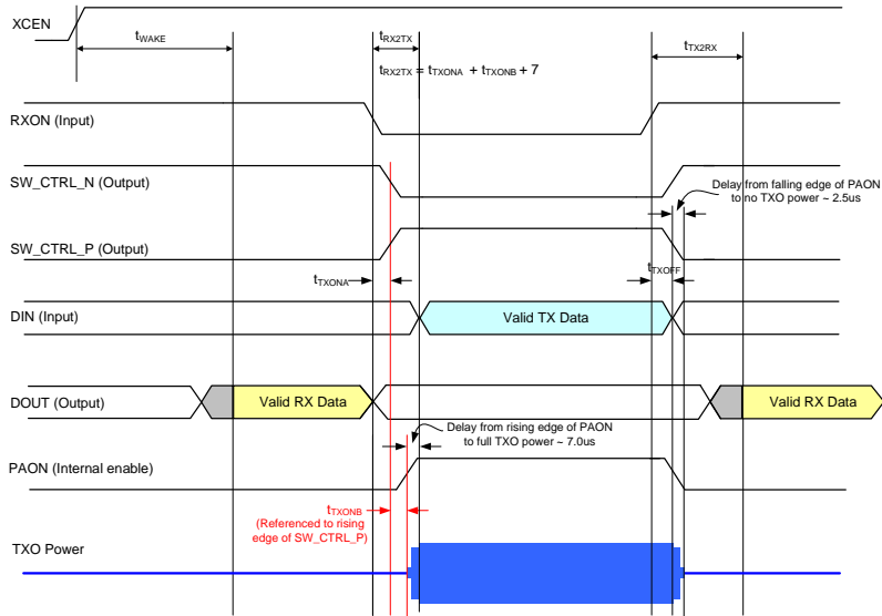
Figure 2a: Control Timing for TDD Operation, PAFIRST=0
