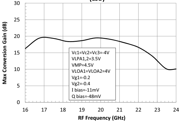
Max Conversion Gain versus RF Frequency (LSB)
