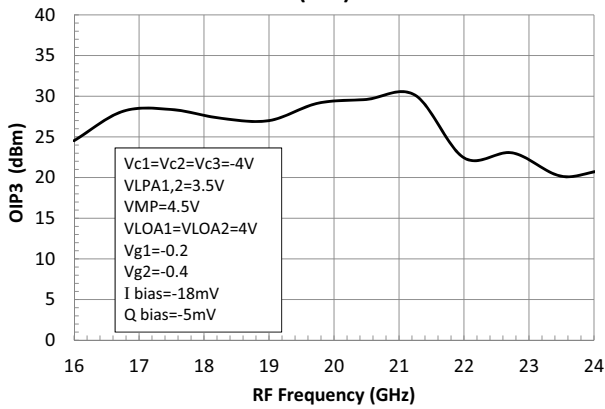
OIP3 versus RF Frequency (LSB)
