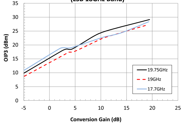
OIP3 versus Conversion Gain (LSB 18GHz Band)
