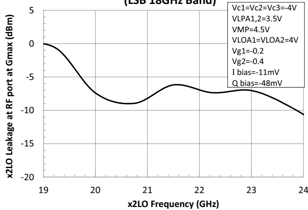
x2LO Leakage at Gmax versus x2LO Frequency (LSB 18GHz Band)
