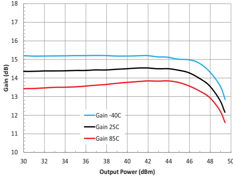
Gain vs. Output Power (f = 2140MHz) (Pulsed 10% duty cycle, 10uS, Vd = 48V, Idq = 300mA)
