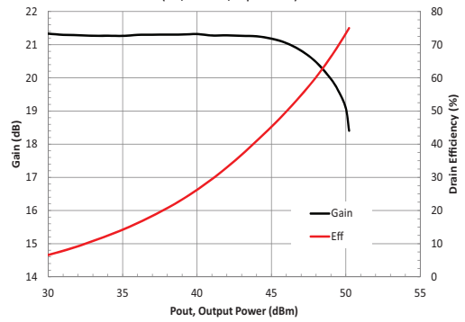
Gain/ Efficiency vs. Pout, f = 900MHz (CW, Vd = 48V, Idq = 300mA)
