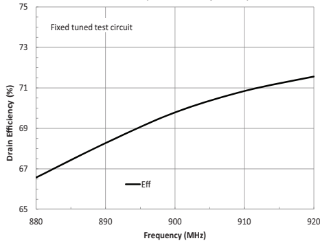
Drain Efficiency vs. Frequency, Pout = 49.5dBm (CW, Vd = 48V, Idq = 300mA)
