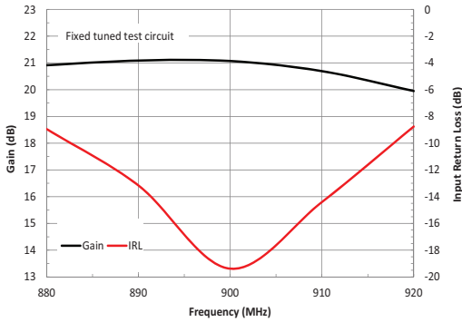
Small Signal Performance vs. Frequency, Pout = 30dBm (Vd = 48V, Idq = 300mA)
