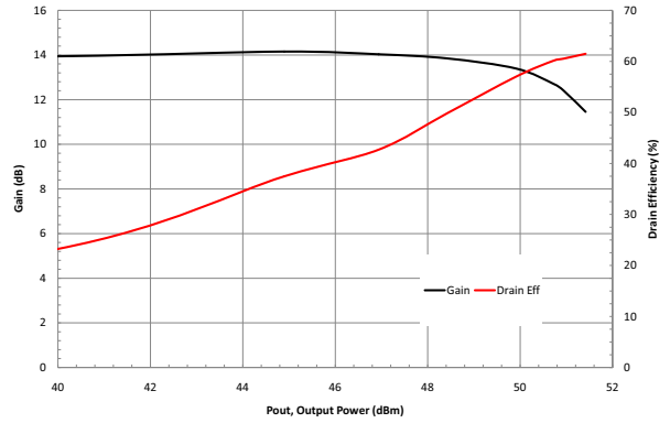
Gain/ Efficiency versus P_{OUT} , F = 2140MHz (Pulsed 10% duty cycle, 10µs, V_D = 48V , I_{DQ} = 440mA )
