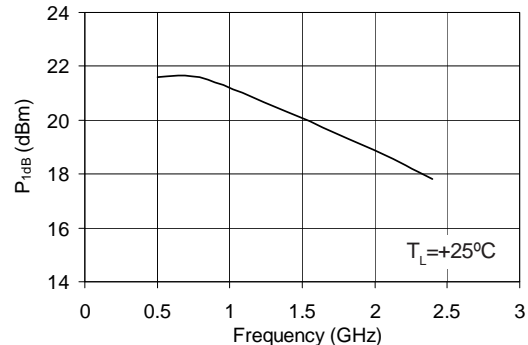
P_{1dB} vs. Frequency V_D = 4.9\text{ V} , I_D = 80\text{ mA}
