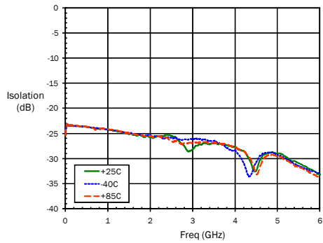
Isolation over Temperature, Max Gain
