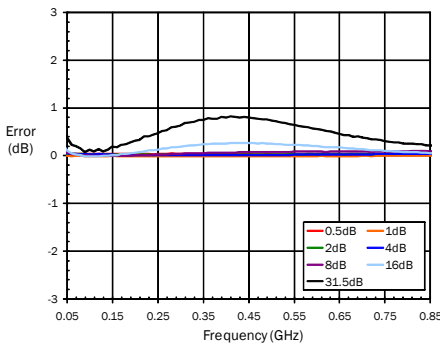
Attenuation Error, Major States, 25C
