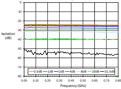
Isolation, Major States, 25C
