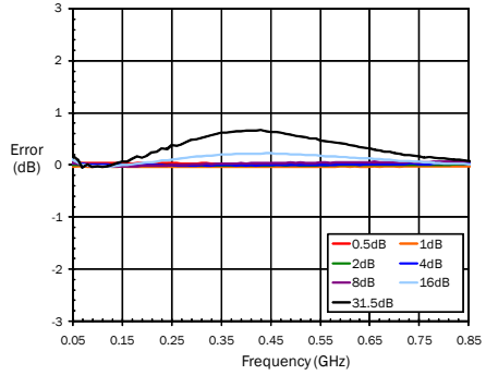
Attenuation Error, Major States, 85C
