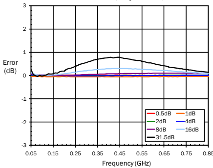
Attenuation Error, Major States, -40C
