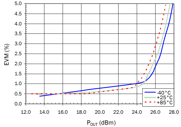
EVM versus P_{OUT} F=2.6GHz 802.11g, OFDM 54Mb/S, 64QAM
