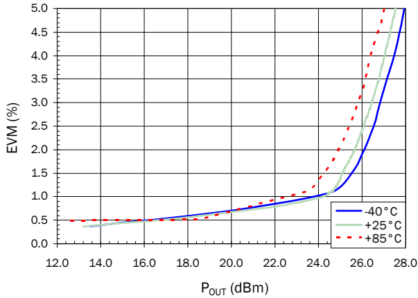
EVM versus P_{OUT} F=2.5GHz 802.11g, OFDM 54Mb/S, 64QAM
