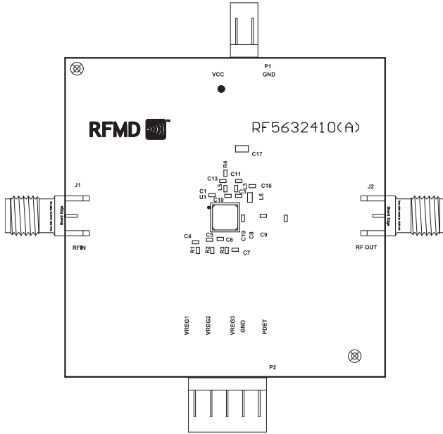
Assembly
