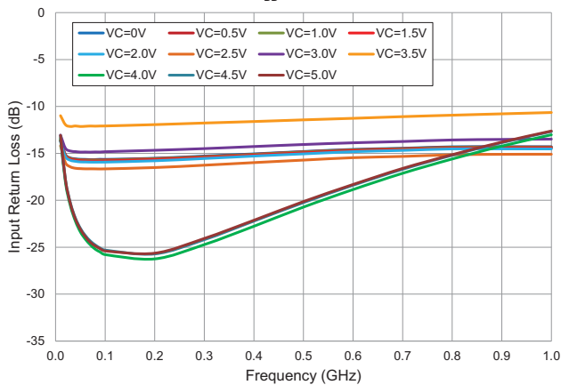
Input Return Loss versus Frequency RFSA3013, V_{DD}=5V , Temp=+25°C
