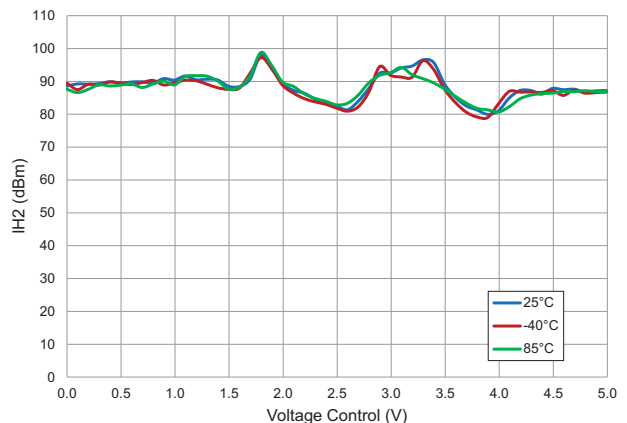
2 nd Harmonic IH2 versus Voltage Control RFSA3013, RF 1GHz, V_{DD}=5V , P_{in}=+15dBm
