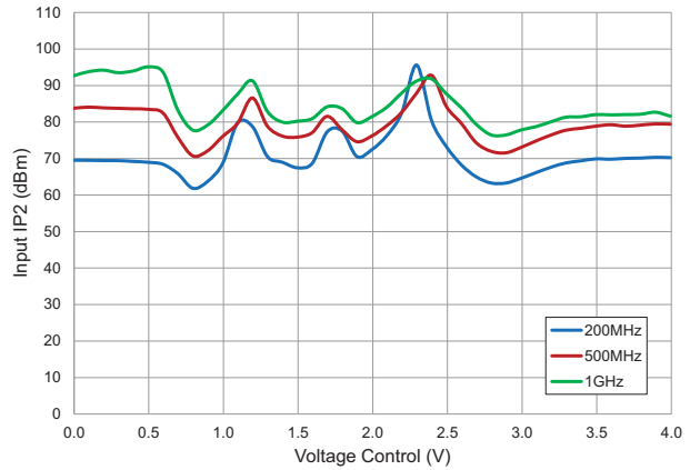
Input IP 2 versus Voltage Control RFSA3013, V DD =5V, Pin=+15dBm/Tone, Temp=+25°C
