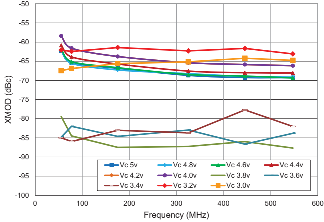
XMOD versus Frequency, 79 Channel 39dBmV Flat Input, Temp=+25°C
