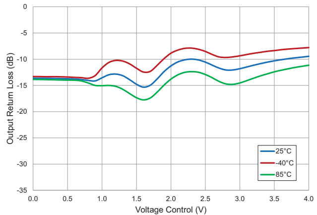
Output Return Loss versus Voltage Control
