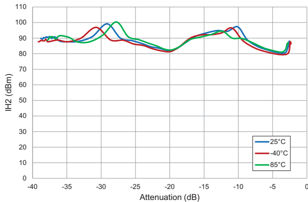
2 nd Harmonic IH 2 versus Attenuation VCA 5V Mode, V DD =5V, F=1GHz Extrapolated from Pin=+15dBm
