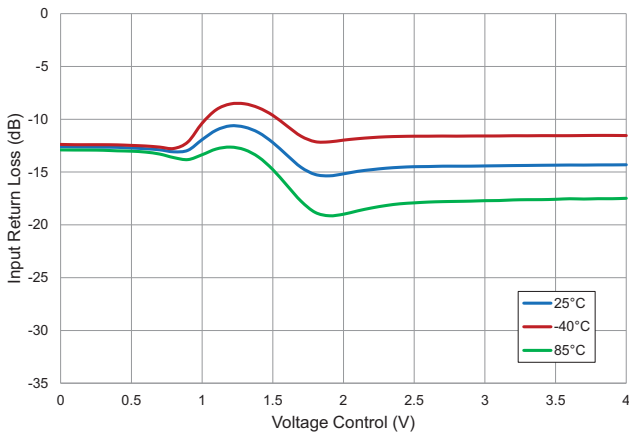
Input Return Loss versus Voltage Control
