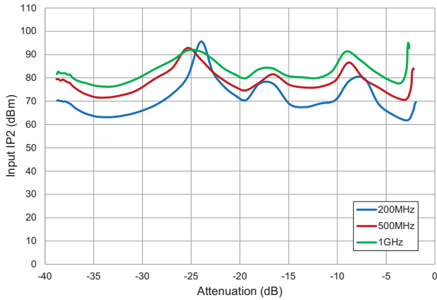
Input IP 2 versus Attenuation RFSA3013, V DD =5V, Pin=+15dBm/Tone, Temp=+25°C
