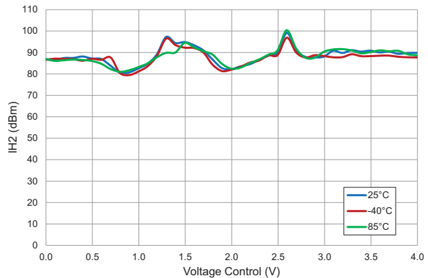
2 nd Harmonic IH 2 versus Voltage Control VCA 5V Mode, V DD =5V, F=1GHz Extrapolated from Pin=+15dBm
