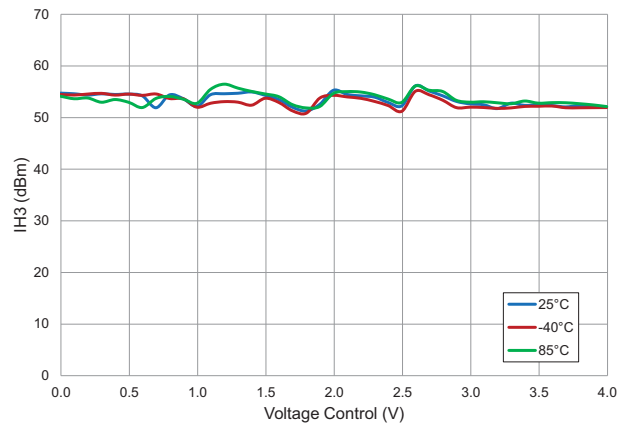
3 rd Harmonic IH 3 versus Voltage Control RFSA3013, RF 1GHz, V DD =5V, Pin=+15dBm
