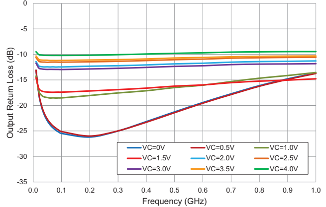
Output Return Loss versus Voltage Control
