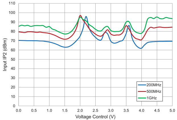
Input IP2 versus Voltage Control RFSA3013, V_{DD}=5V , P_{in}=+15dBm/Tone , Temp=+25^{\circ}C
