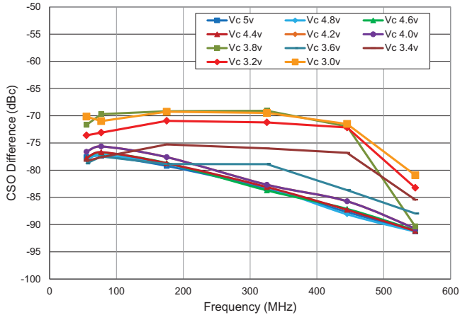
CSO Difference versus Frequency, 79 Channel 39dBmV Flat Input, Temp=+25°C
