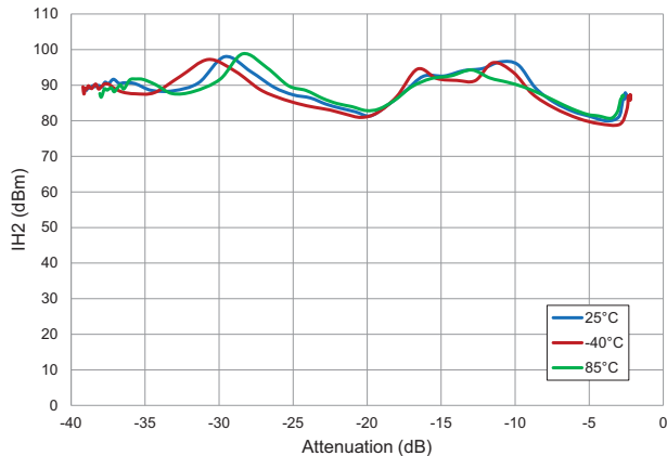
2 nd Harmonic IH2 versus Attenuation RFSA3013, RF 1GHz, V_{DD}=5V , P_{in}=+15dBm
