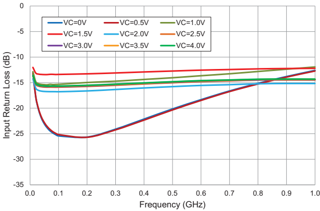
Input Return Loss versus Voltage Control
