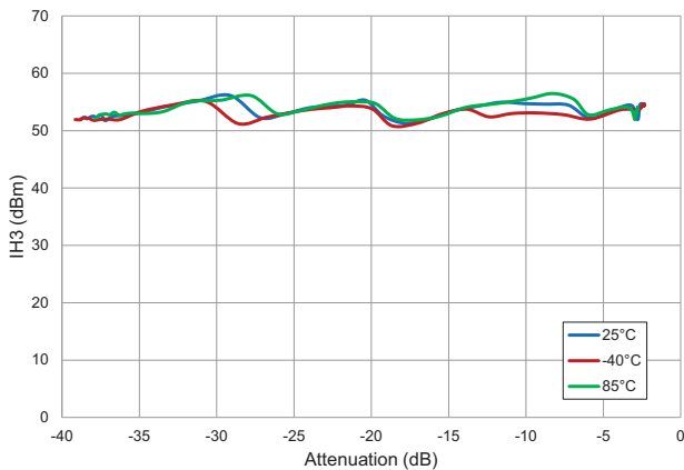
3 rd Harmonic IH 3 versus Attenuation RFSA3013, RF 1GHz, V DD =5V, Pin=15dBm
