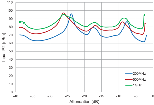
Input IP2 versus Attenuation RFSA3013, V_{DD}=5V , P_{in}=+15dBm/Tone , Temp=+25^{\circ}C
