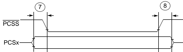
Figure 38. DSPI PCS strobe (PCSS) timing
