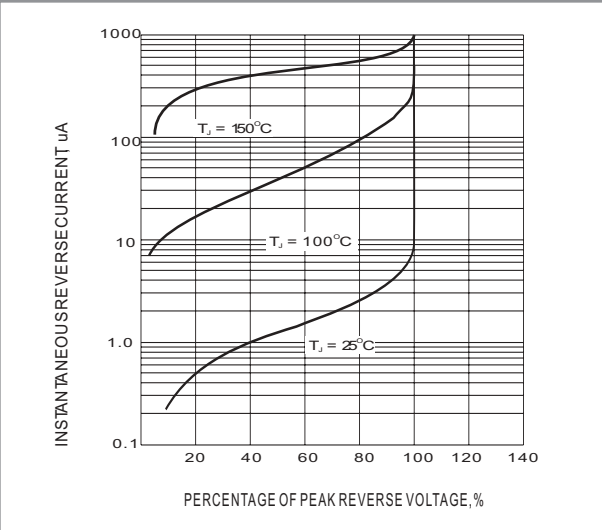
Fig.4-TYPICAL REVERSE CHARACTERISTIC
