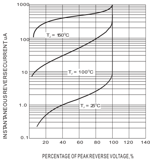
Fig.3 TYPICAL REVERSE CHARACTERISTIC
