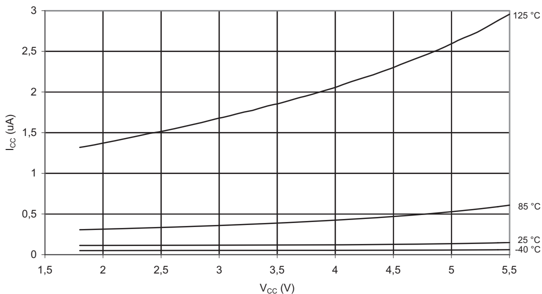
Figure 2-8. Power-down Supply Current vs. V_{CC} (Watchdog Timer Enabled)
