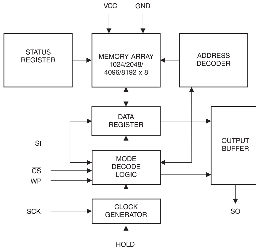
Figure 1-1. Block Diagram
