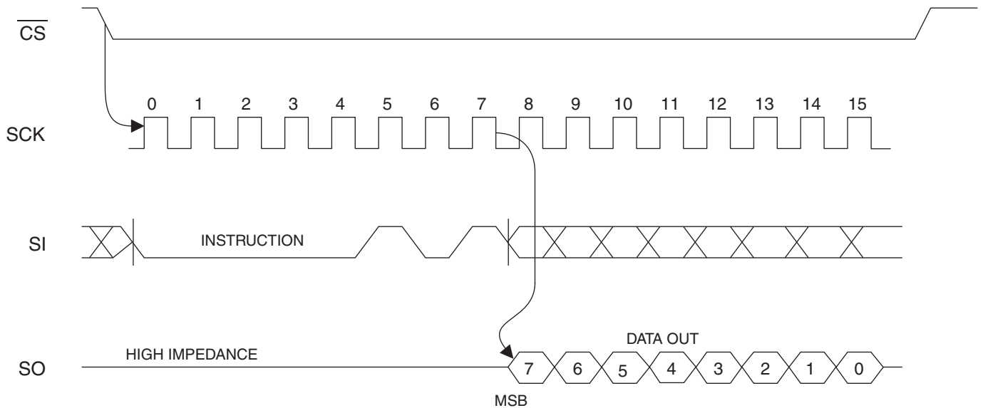
Figure 4-4. RDSR Timing
