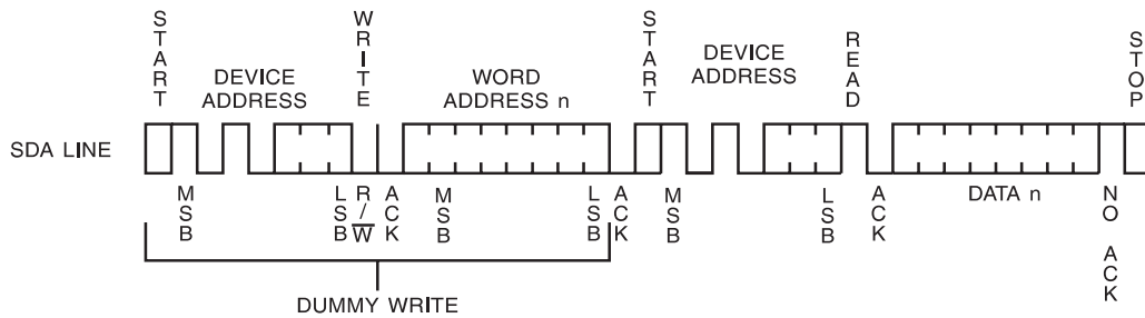
Figure 14. Random Read
