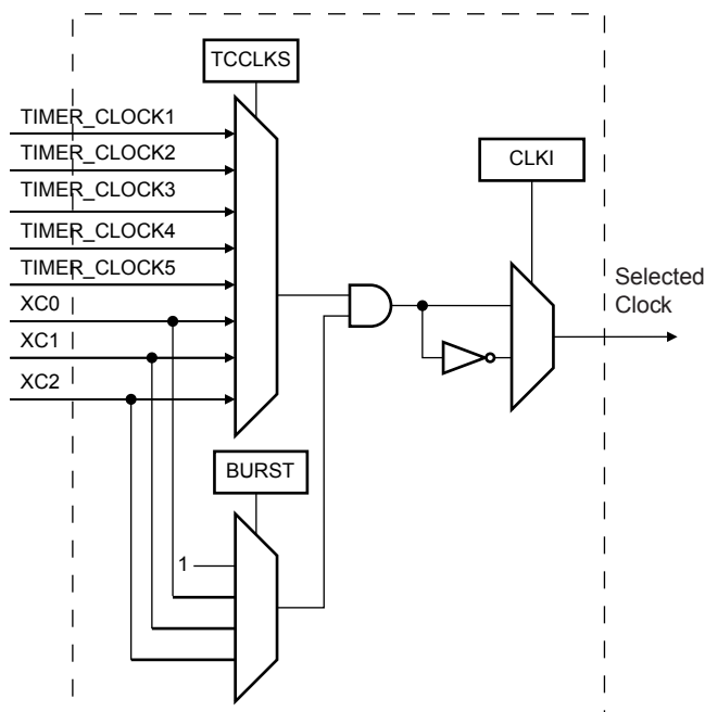
Figure 31-2. Clock Selection
