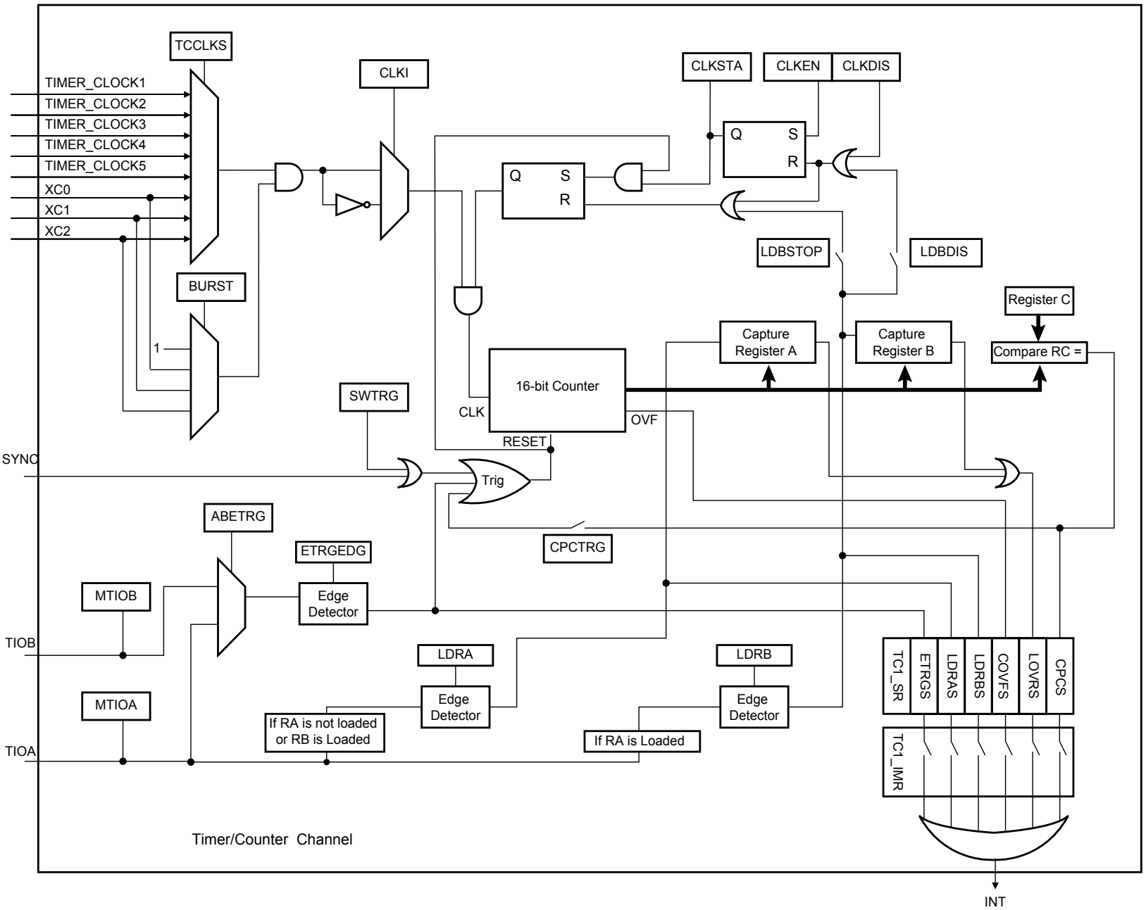
Figure 31-4. Capture Mode
