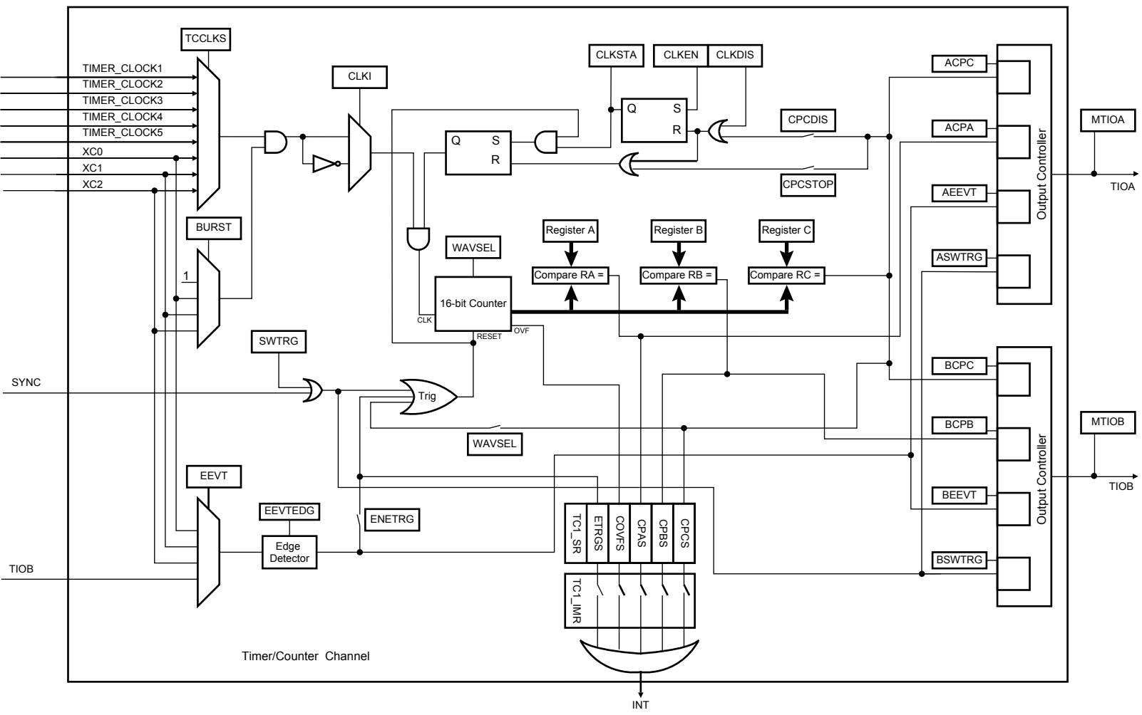
Figure 31-5. Waveform Mode
