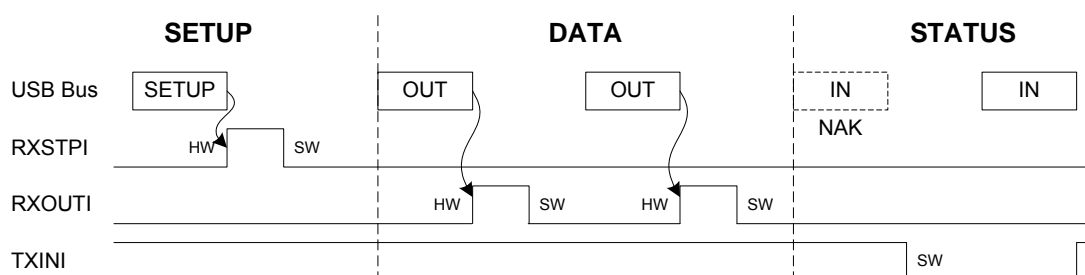
Figure 30-15. Control Write
