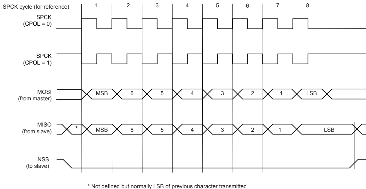
Figure 23-4. SPI Transfer Format (NCPHA = 0, 8 bits per transfer)
