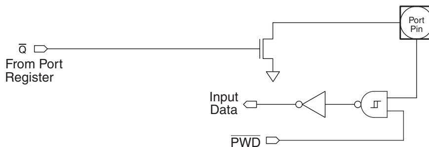
Figure 10-4. Open-drain Output
