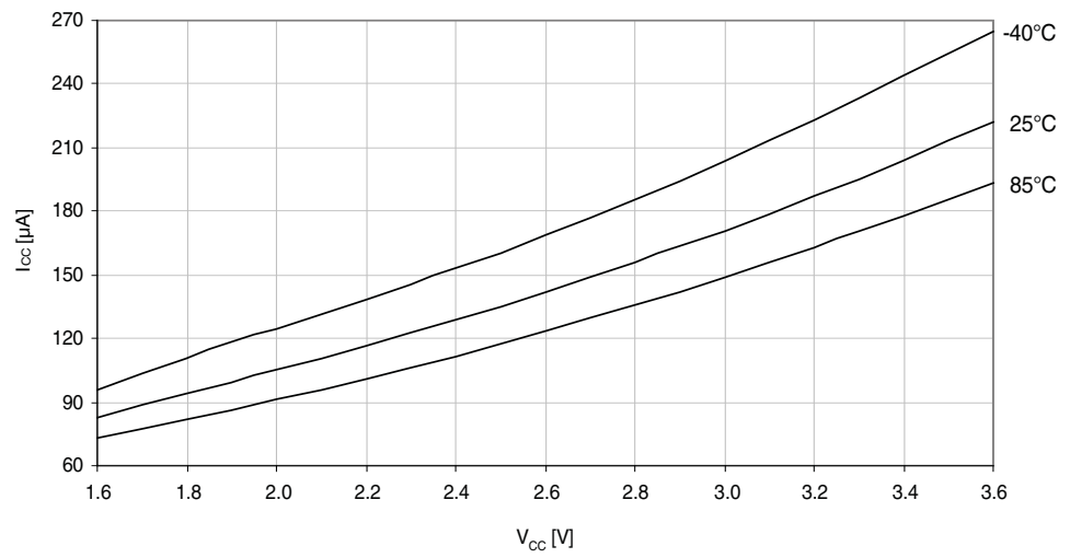
Figure 33-3. Active mode supply current vs. V_{CC} .
