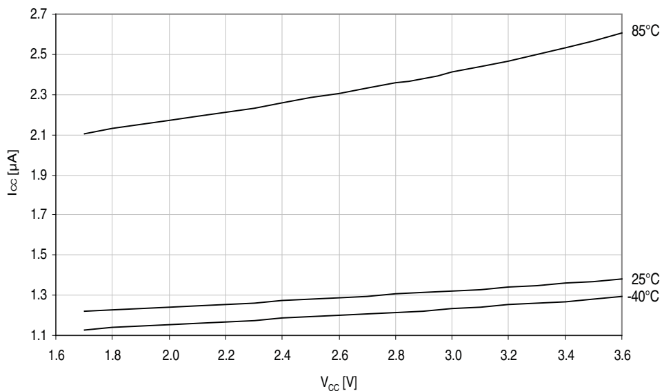
Figure 33-17. Power-down mode supply current vs. V_{CC} . Watchdog and sampled BOD enabled.
