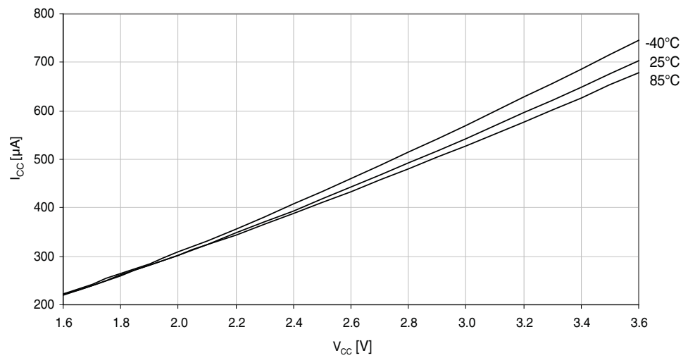
Figure 33-4. Active mode supply current vs. V_{CC} .
