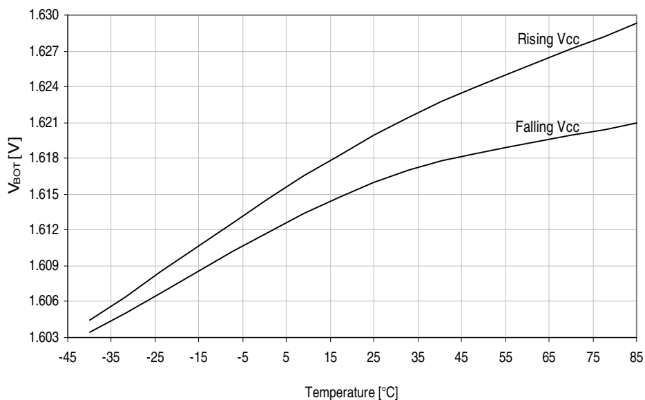
Figure 33-42. BOD thresholds vs. temperature.
