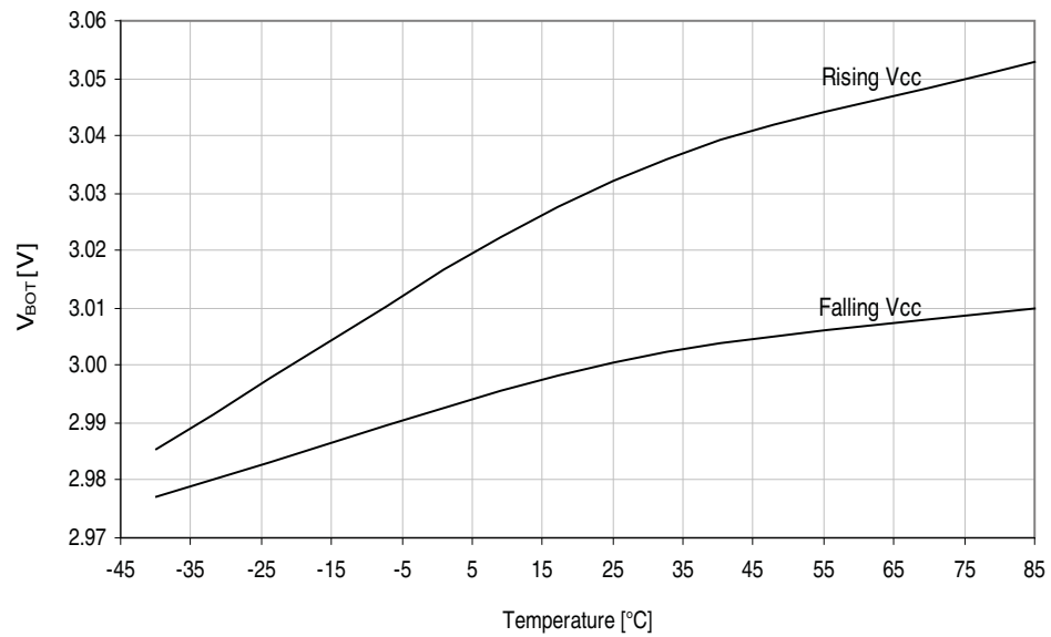
Figure 33-43. BOD thresholds vs. temperature.
