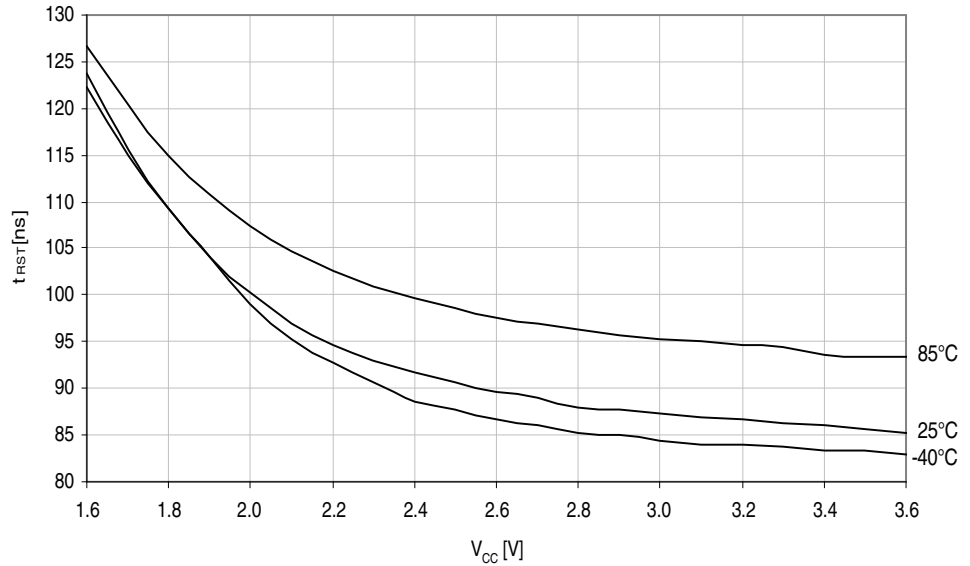
Figure 33-44. Minimum reset pin pulse width vs. V CC .
